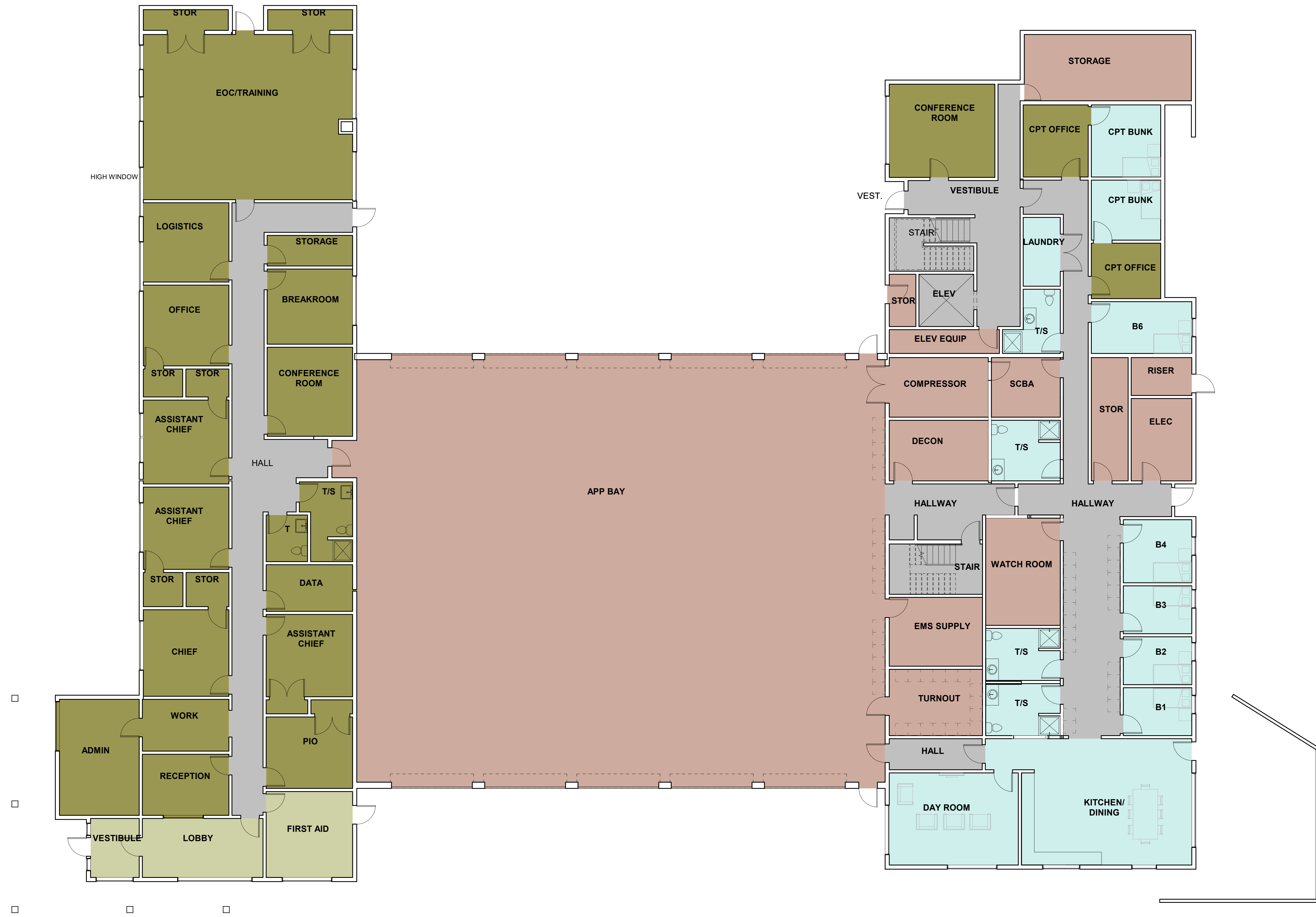
1 A2.1 FIRST FLOOR PLAN-ORIGINAL WITH MINOR COMMENTS A1.10A 1/8" = 1'-0"
